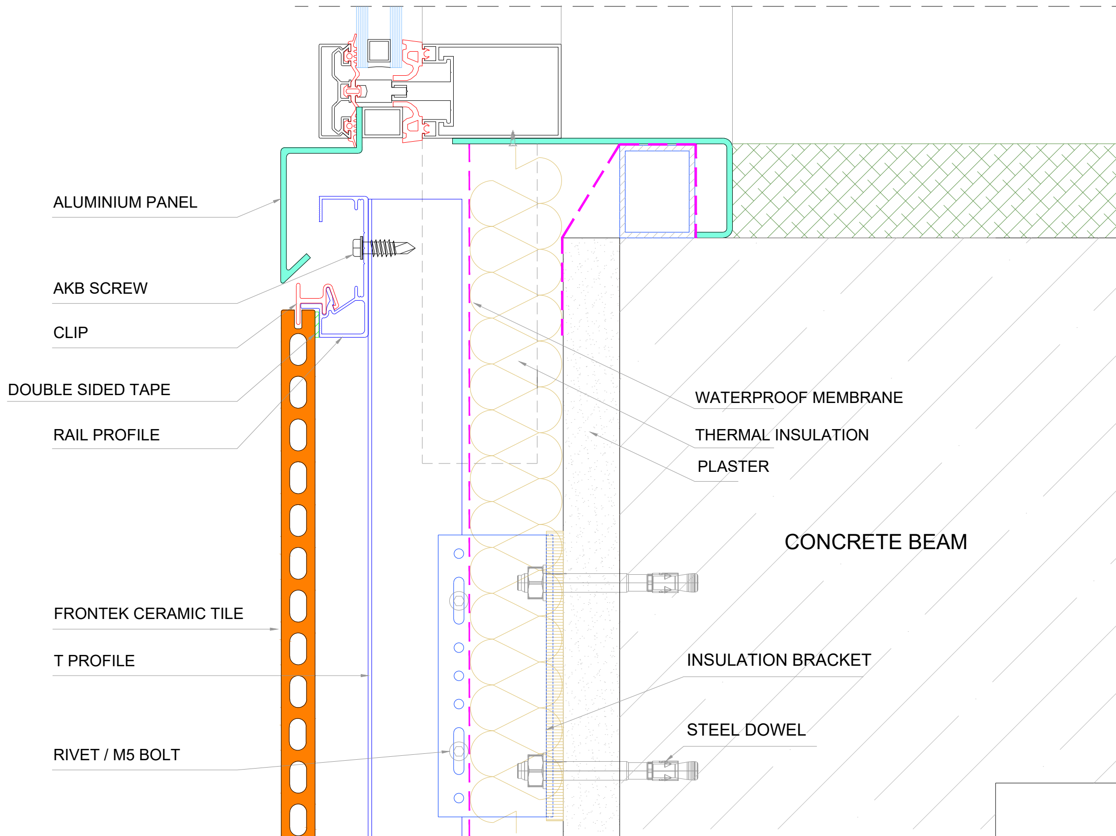
DETAIL C
