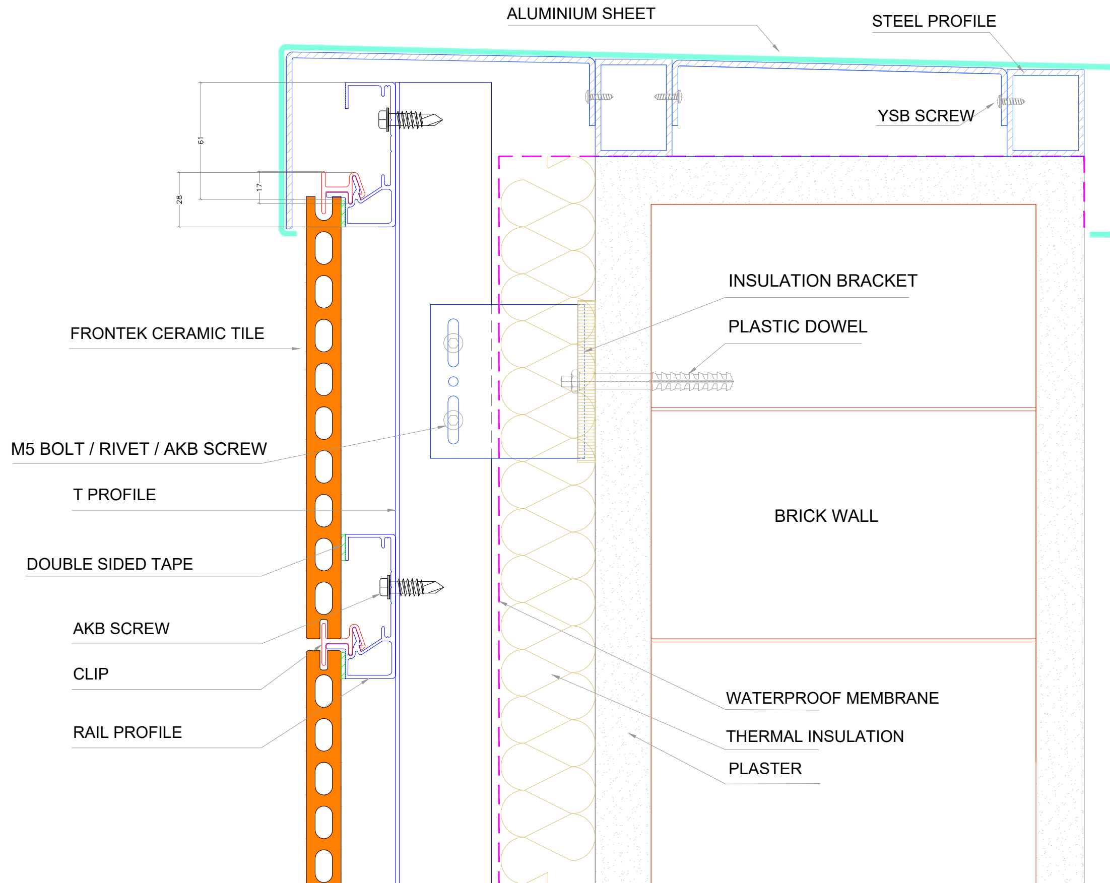
DETAIL 6
