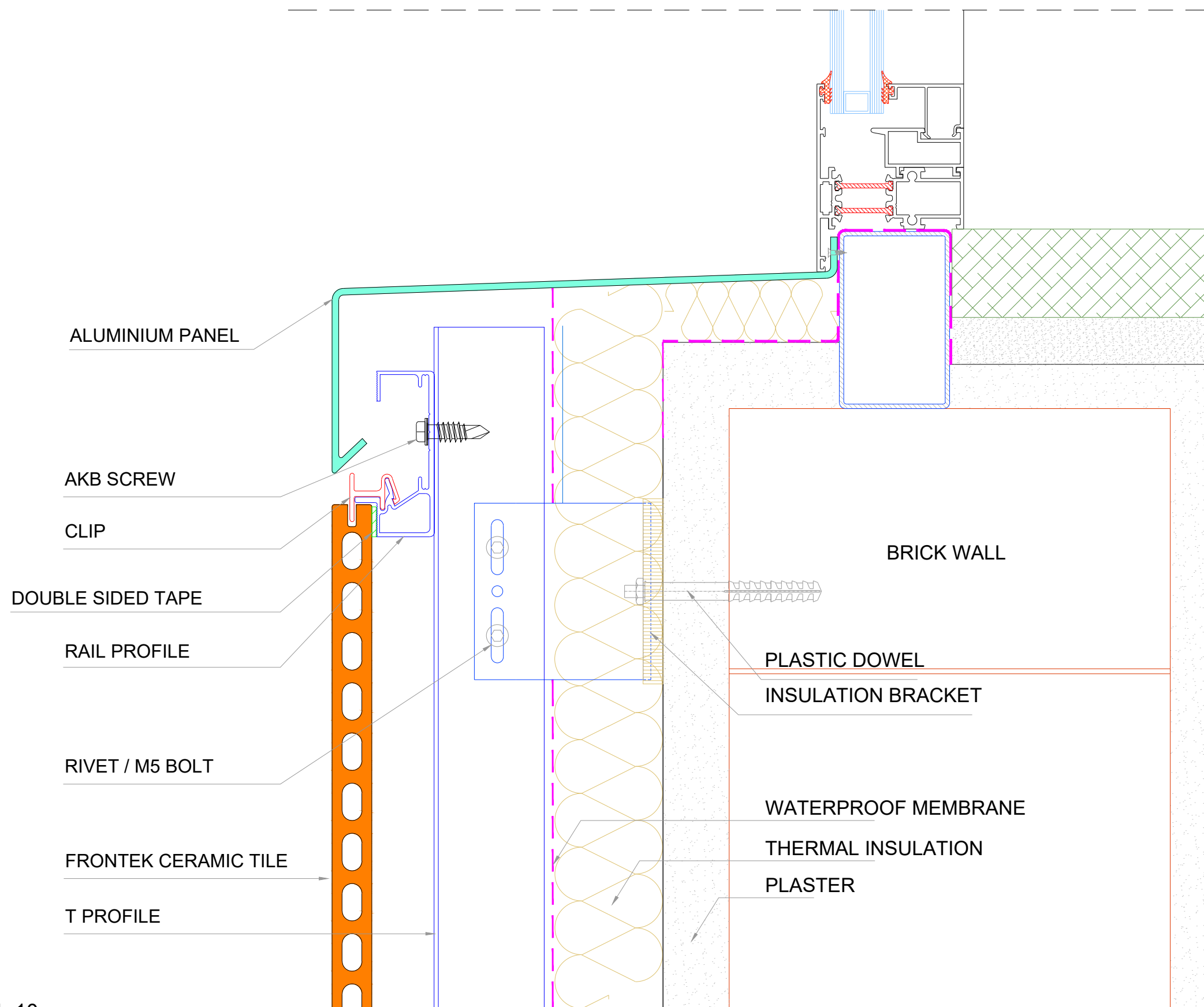
DETAIL 10
