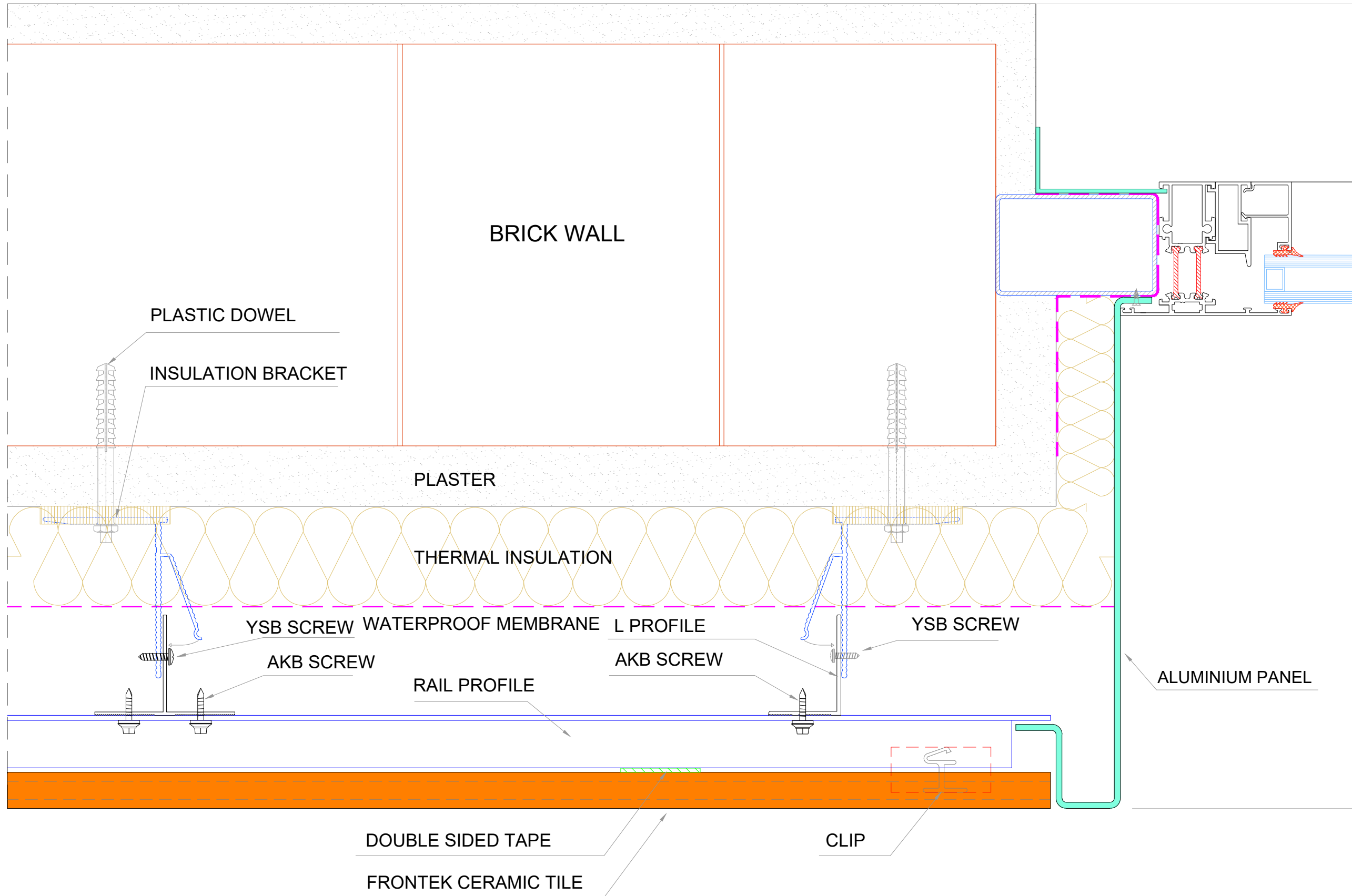
DETAIL 8
